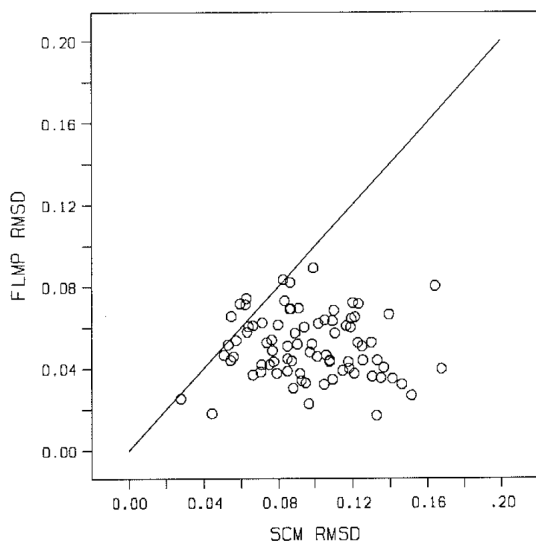
Figure 1. The RMSD value for the fit of the FLMF on the ordinate as a function on the RMSD value for the single channel model on the abscissa for each of the 82 subjects in the database [5].
