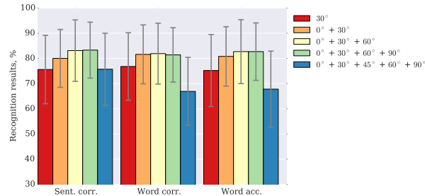
Figure 1: Best mean recognition results (in %) across test subjects for each number of views per combination of the OuluVS2 short phrase multi-view dataset using the proposed method.
